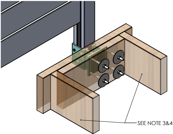
DECK SURFACE HIDDEN FOR CLARITY
