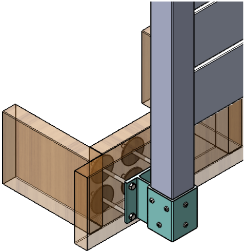
DECK SURFACE HIDDEN FOR CLARITY
