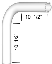
90° Handrail extension
