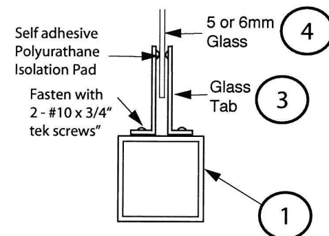
Aluminum Glass Tab Detail
