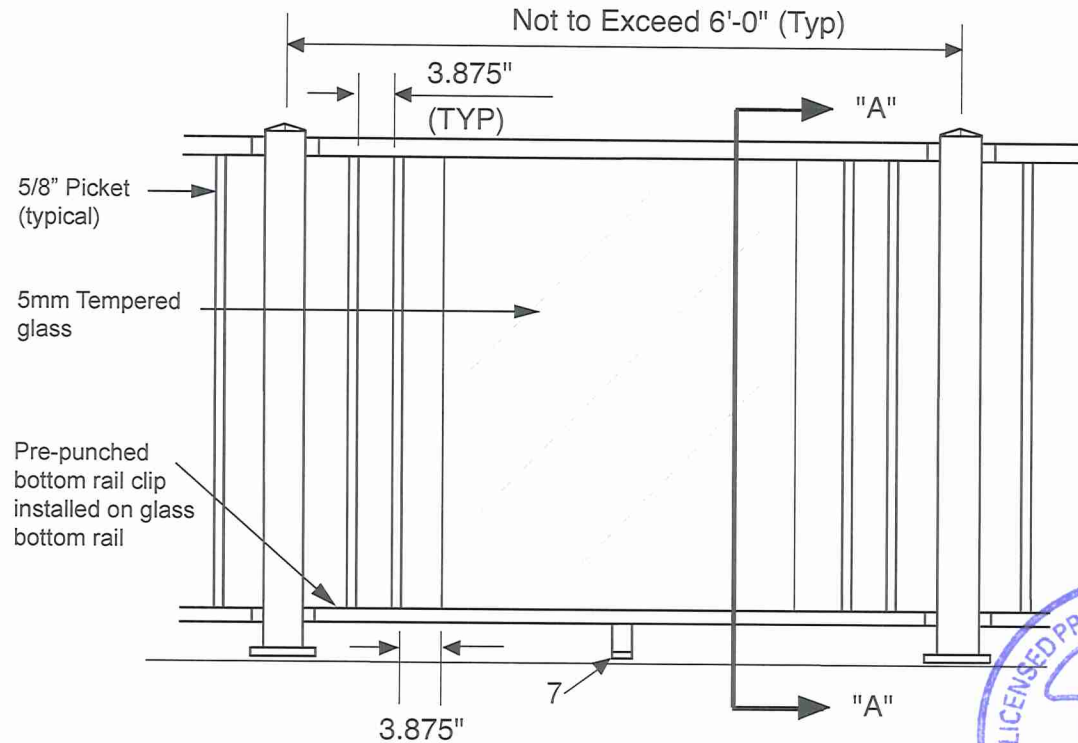
ELEVATION OF BALCONY RAILING NOT TO SCALE
