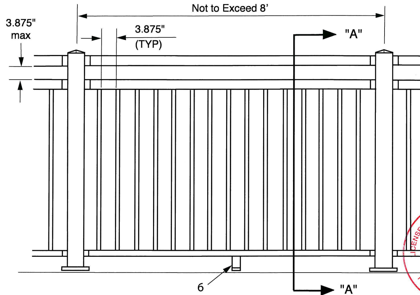
ELEVATION OF BALCONY RAILING NOT TO SCALE
