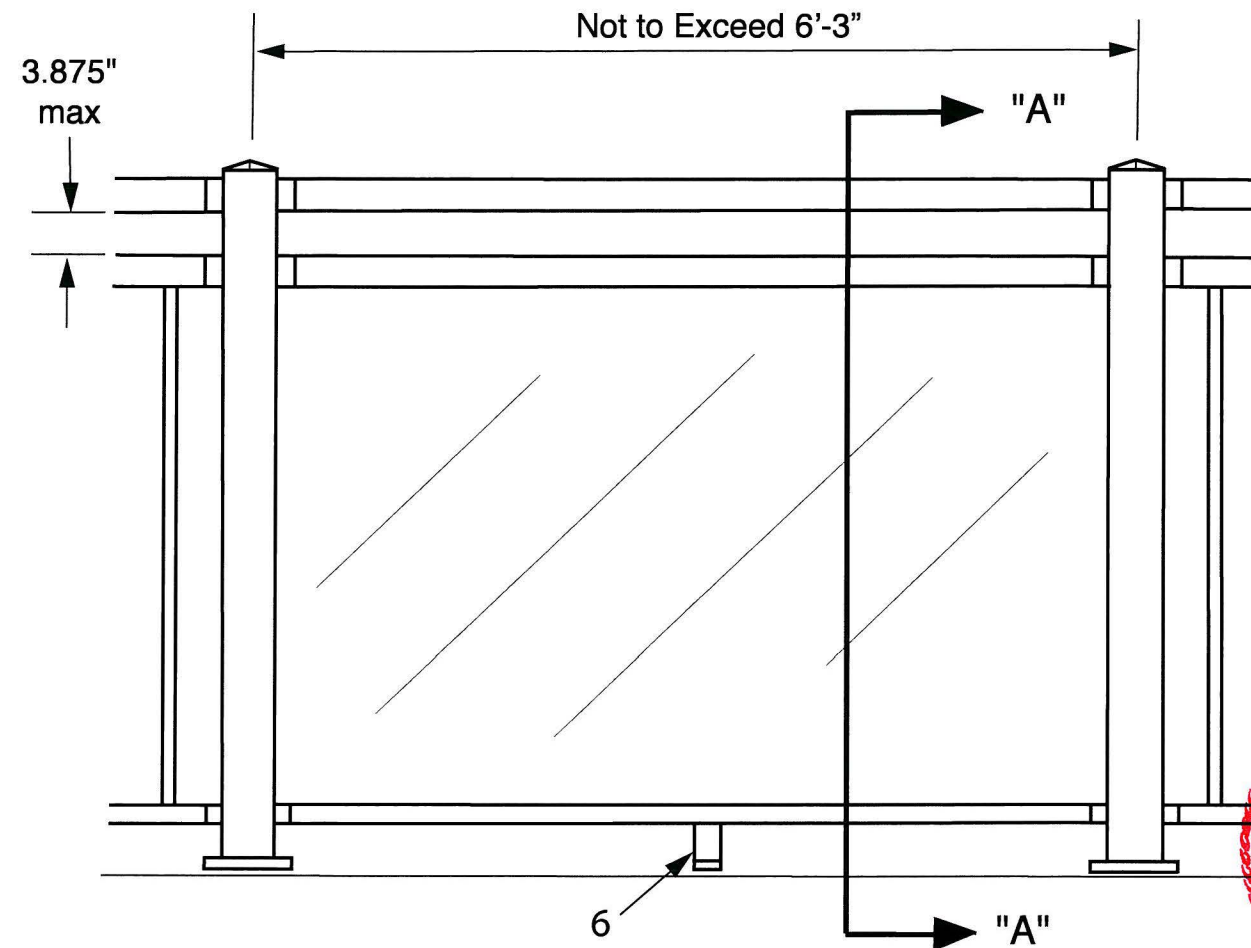
ELEVATION OF BALCONY RAILING NOT TO SCALE
