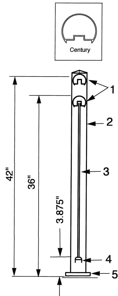
SECTION "A-A" NOT TO SCALE
