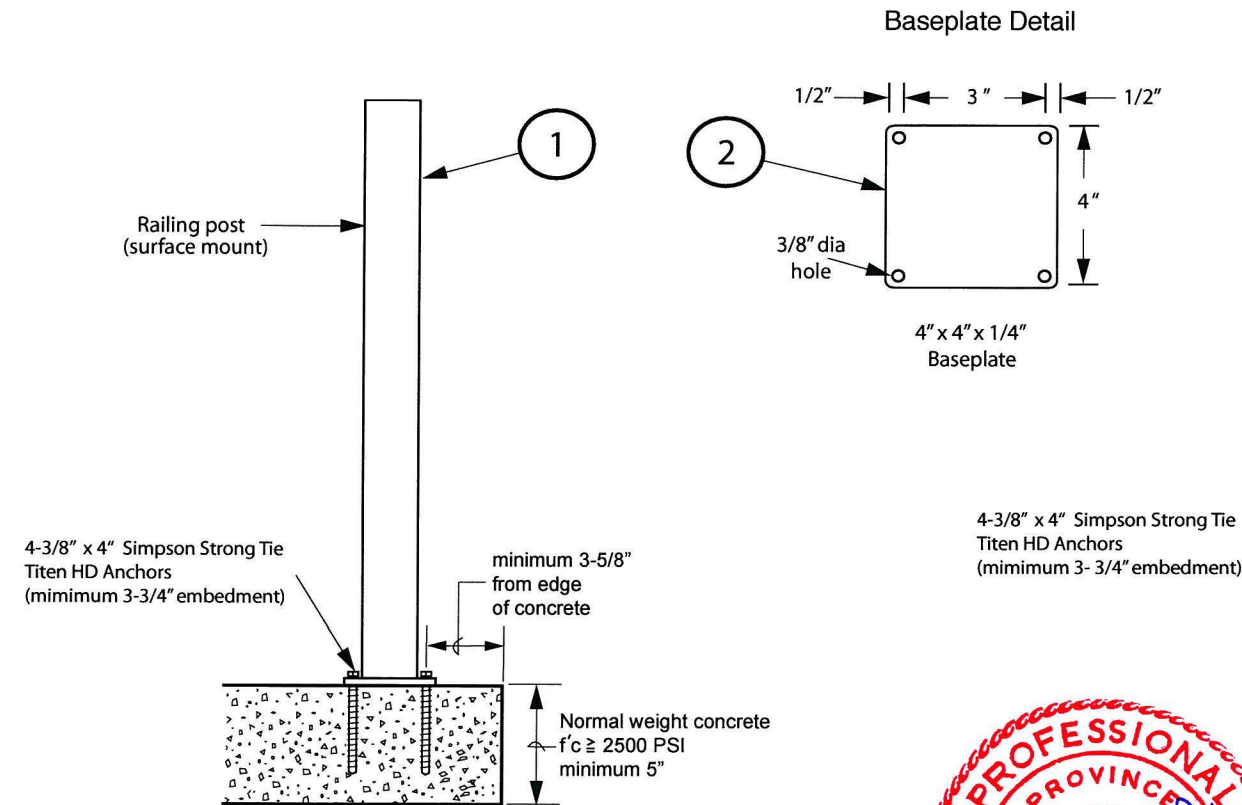
Typical Post to Concrete Install
